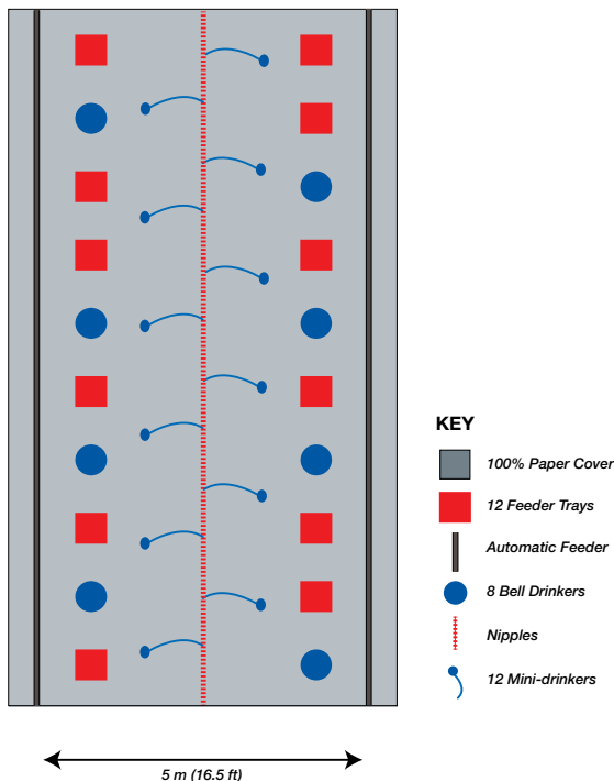
Figure 13: Typical whole-house brooding layout for 1,000 chicks.
