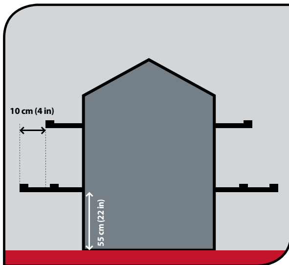
Figure 53: Manual nest box set-up.
