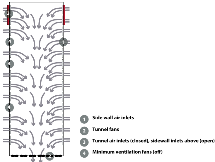
Figure 111: Typical air movement during transitional ventilation.
