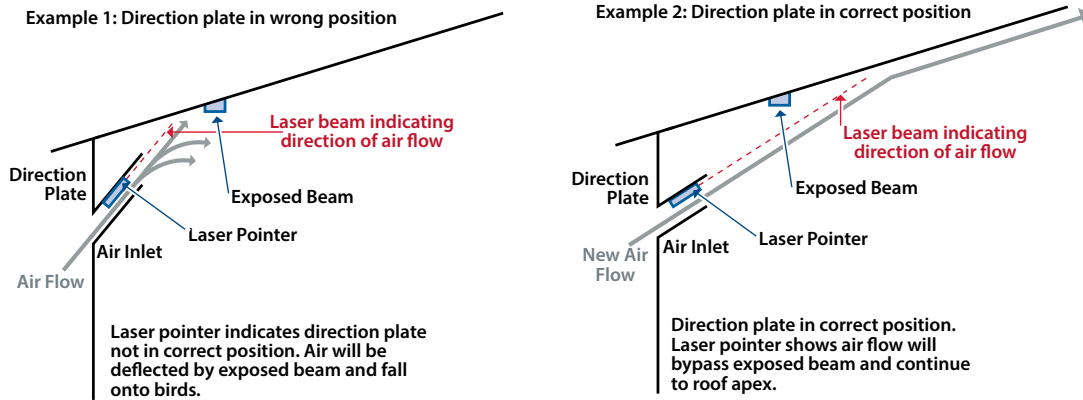
Figure 107: Using a presentation laser to determine if the air direction plate is positioned correctly. A simple laser pointer can be used to provide a visual reference of direction of air flow into the house. The direction plate can then be set to ensure that air flow bypasses any ceiling obstructions.
