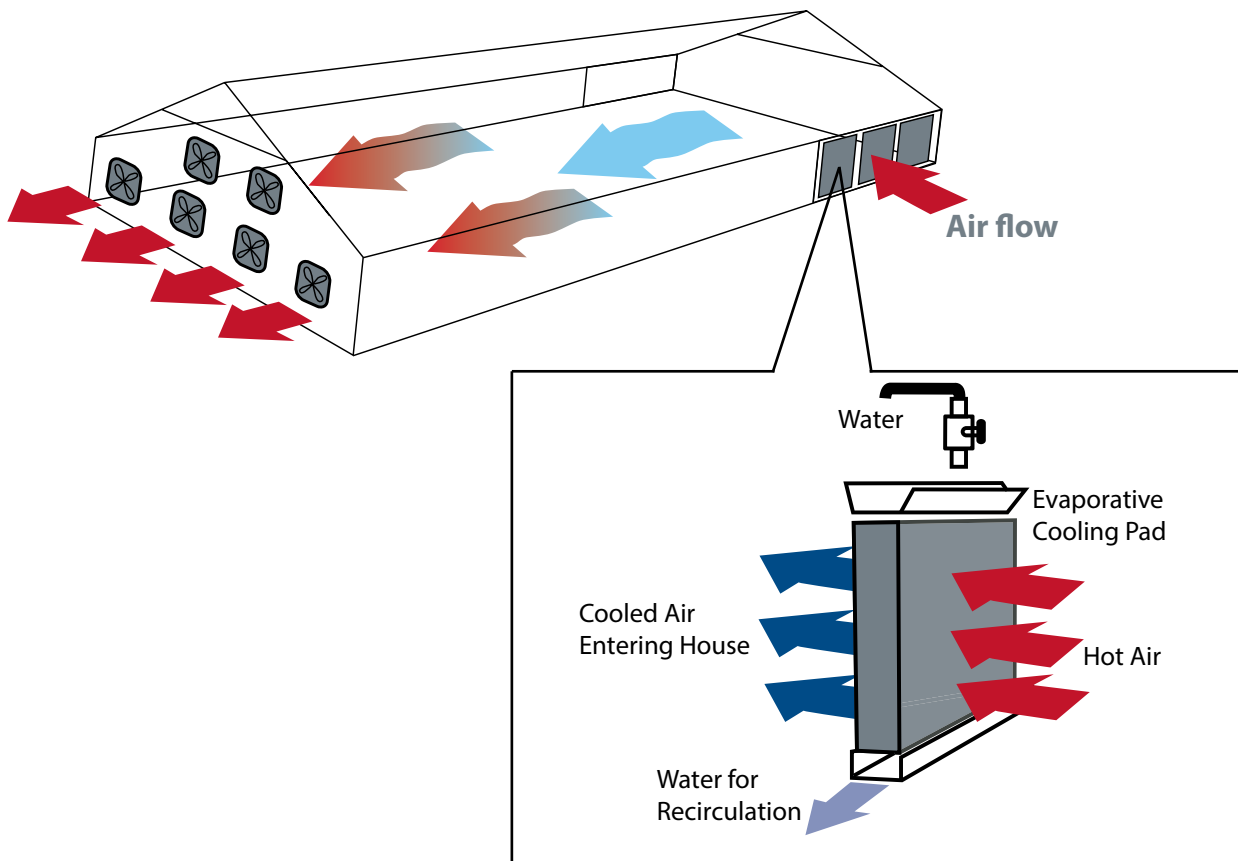
Figure 117: Pad cooling with tunnel ventilation.
