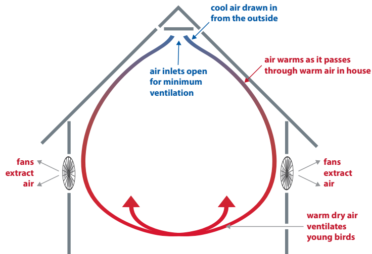
Figure 110: Diagram of reverse flow (roof inlet) ventilation.
